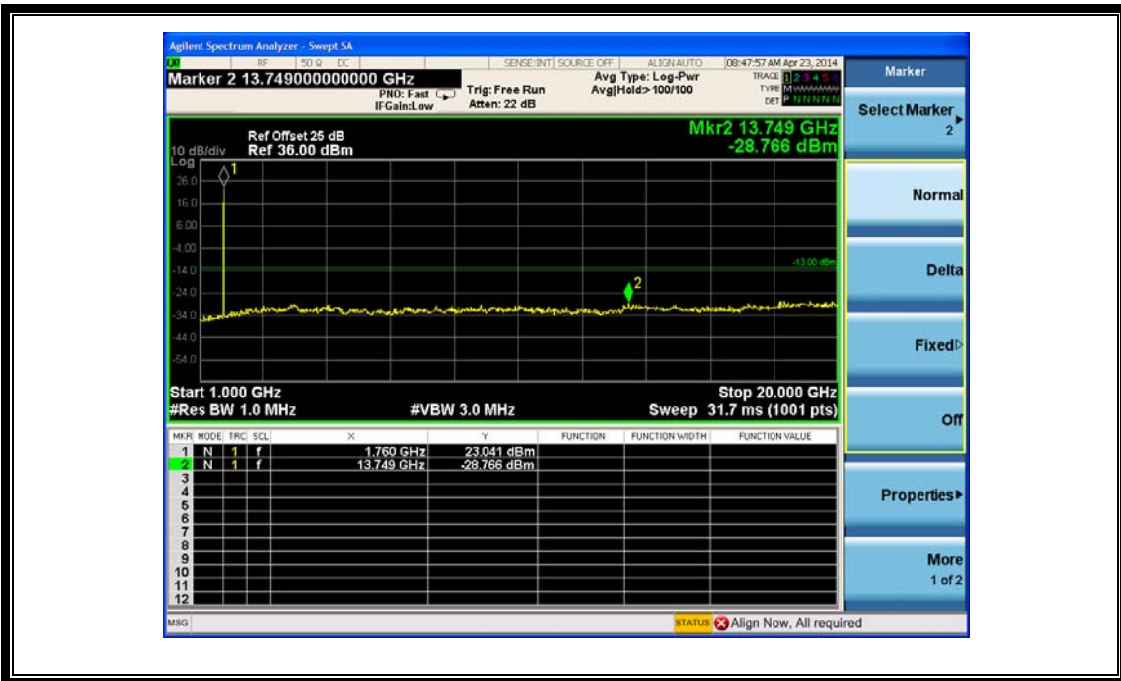
(Plot P3.1: HSPA+1700MHz Channel = 1513 1GHz to 20GHz)
