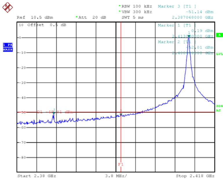
Band Edge, Left Side
