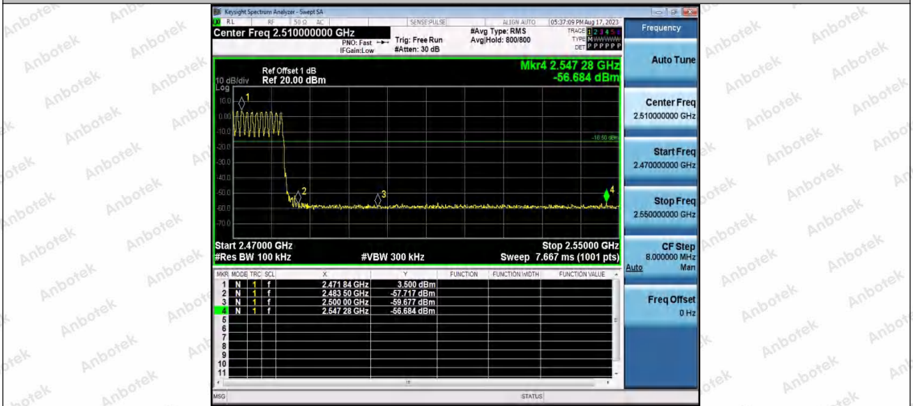
2.4G_Ant1_High_Hop_2480
