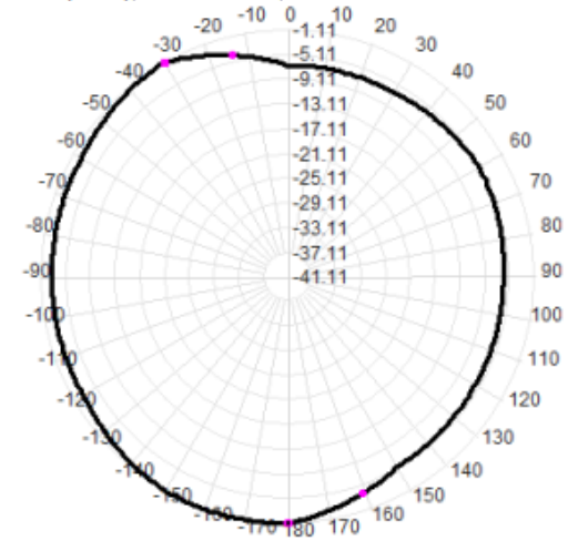
Total(H-XY), Max=-1.11dBi, CirD=5.78
