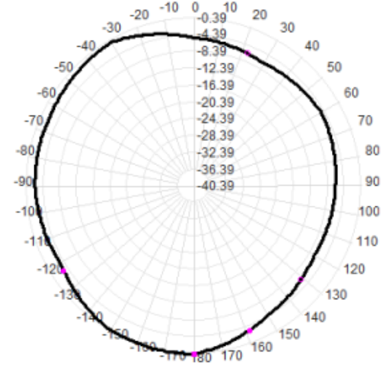
Total(H-XY), Max=-0.44dBi, CirD=6.89
