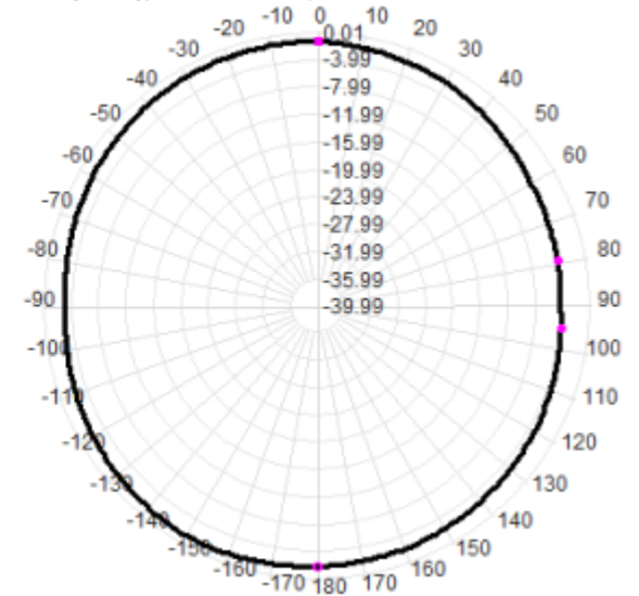
Total(H-XY), Max=-1.32dBi, CirD=3.20
