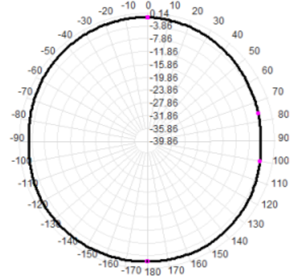
Total(H-XY), Max=-1.09dBi, CirD=3.42
