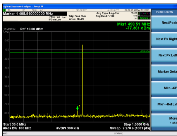
TX CH48(30MHz-1GHz)
