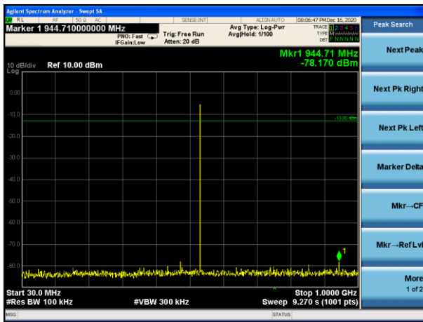
TX CH48(30MHz-1GHz)
