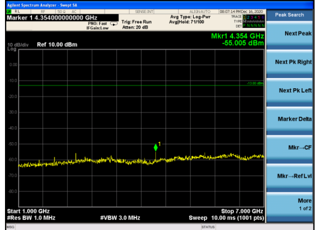
TX CH48(1GHz-7GHz)
