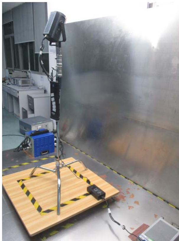
Conducted Emissions Side – VL300 View
