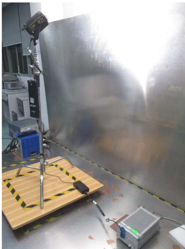
Conducted Emissions Side –VL200 View
