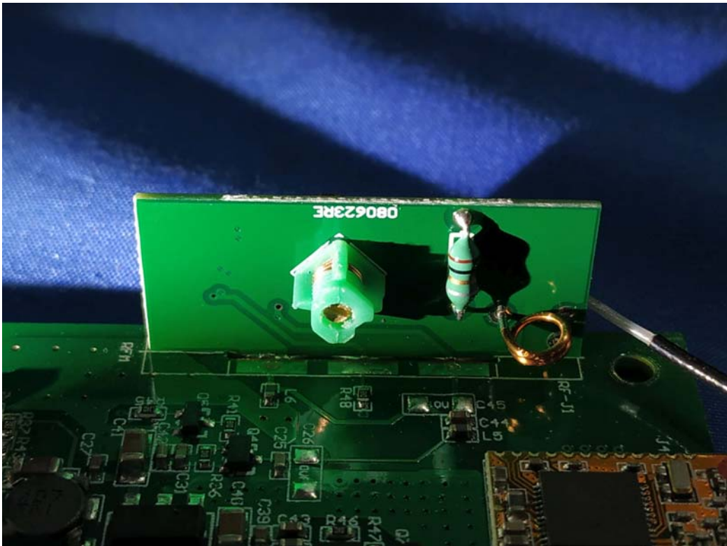
2.4G SRD Receiver module rear
