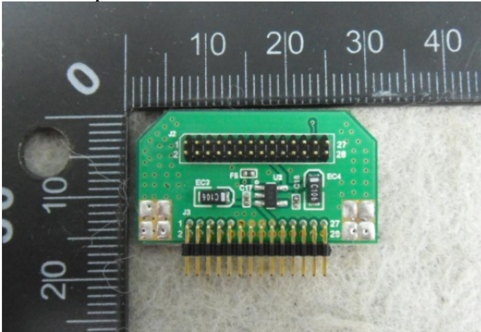
- HD-CIS-IF Board Top
