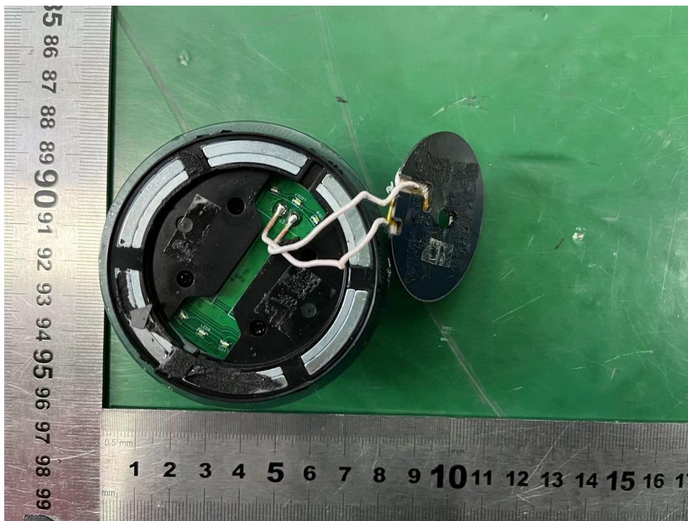
Inductive Loop Antenna
