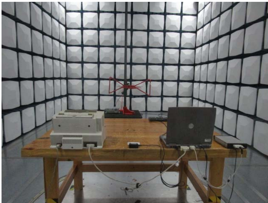
Radiated Emissions –Rear View (Below 1GHz) For USB
