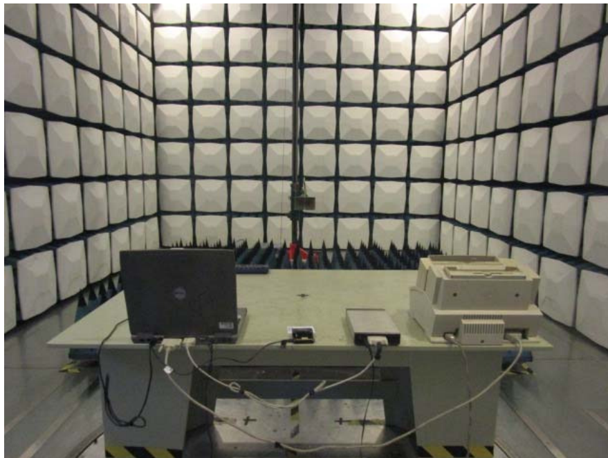
Radiated Emissions –Rear View (Above 1GHz) For USB
