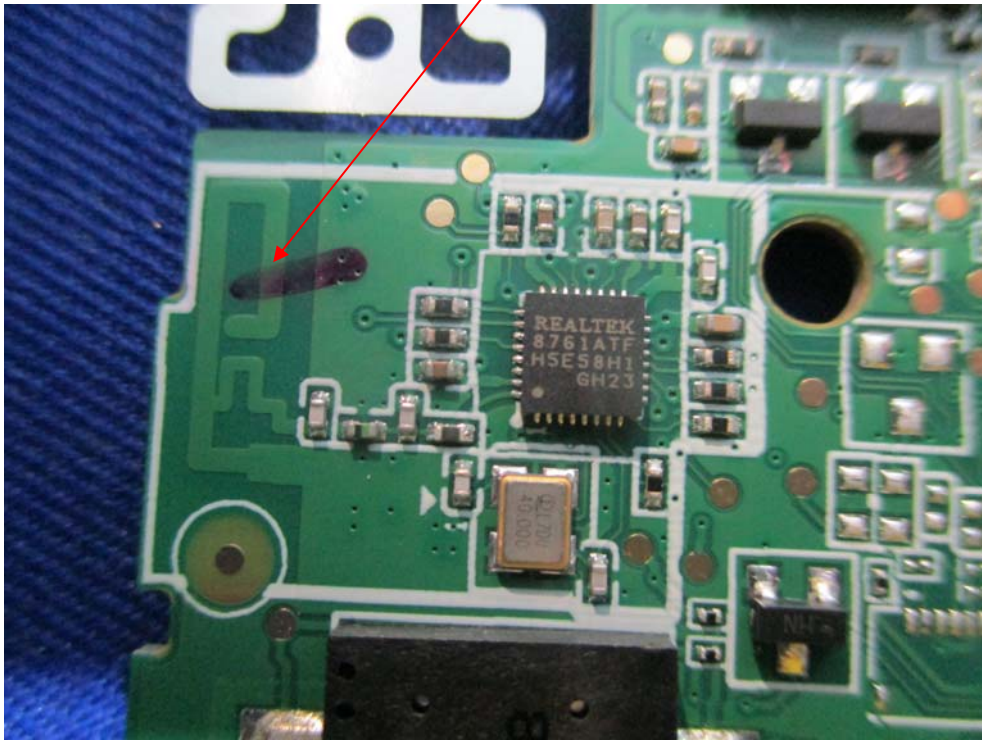
Bluetooth ANT
