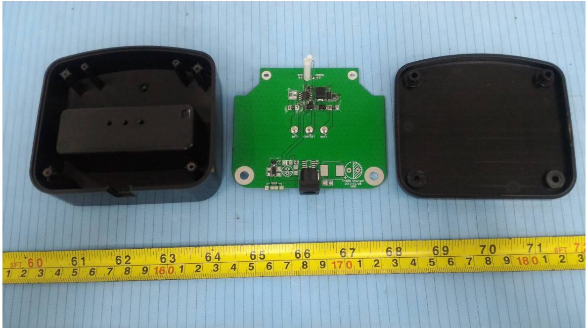
EUT – Cover off View (Charger)
