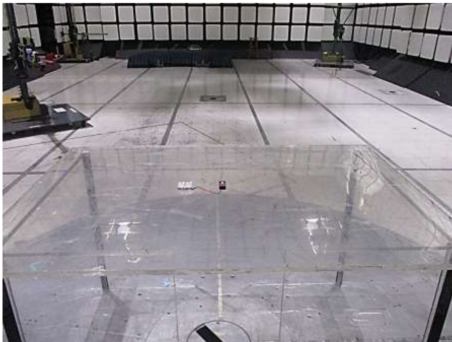
Photograph 2. Radiated Emissions, (30 MHz – 1000 MHz), Rear View
