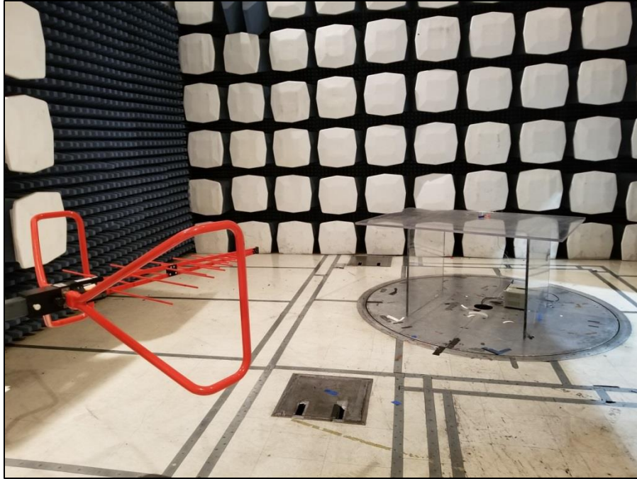
Photograph 3. Radiated Spurious Emissions, Below 1 GHz, Test Setup
