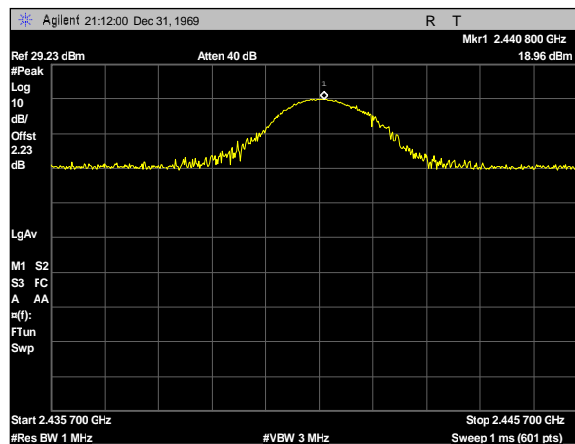
Plot 16. Peak Power Output, 18.96dBm, Mid
