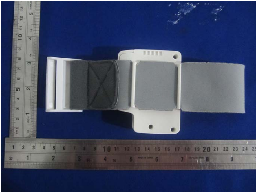
EUT—Bottom View
