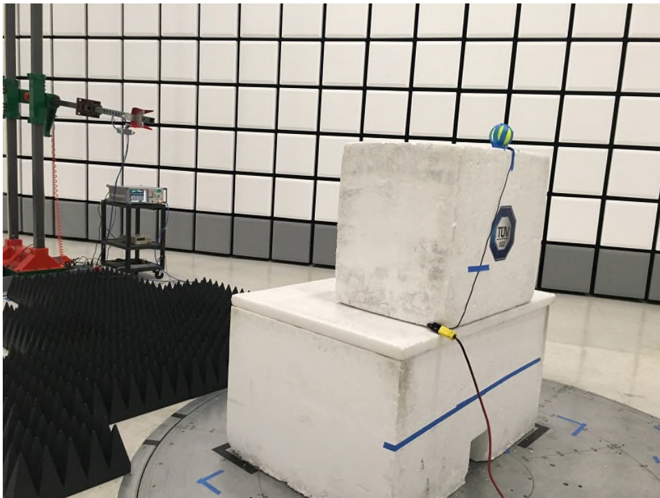
Radiated Spurious Emissions Above 1GHz 1GHz Rear (Softball Transmit Mode)
