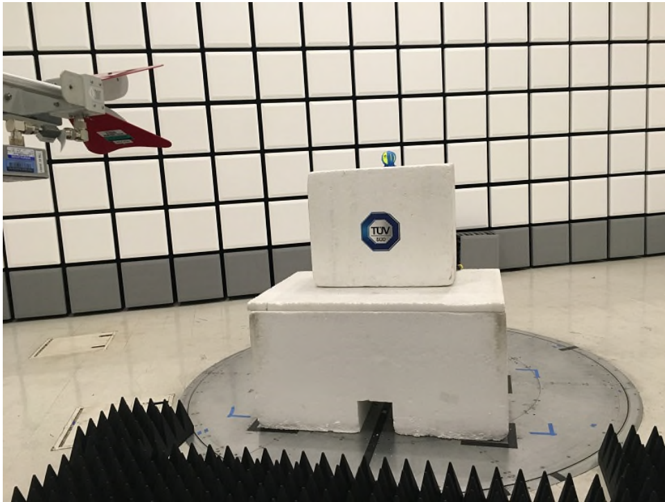
Radiated Spurious Emissions Above 1GHz Front (Softball Transmit Mode)
