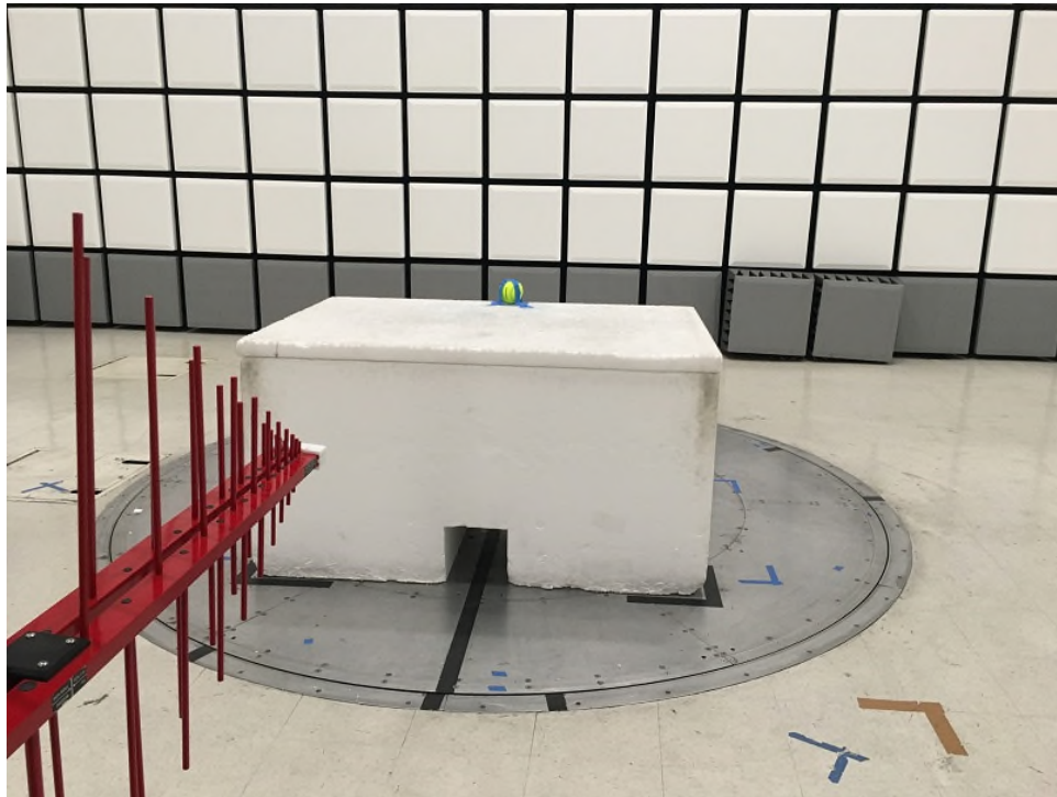
Radiated Spurious Emissions Below 1GHz Front (Softball Transmit Mode)
