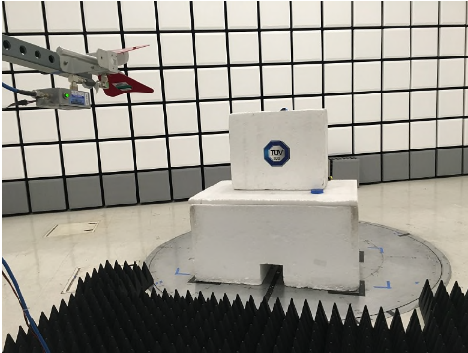
Radiated Spurious Emissions Above 1GHz Front (Swing tracker Transmit Mode)
