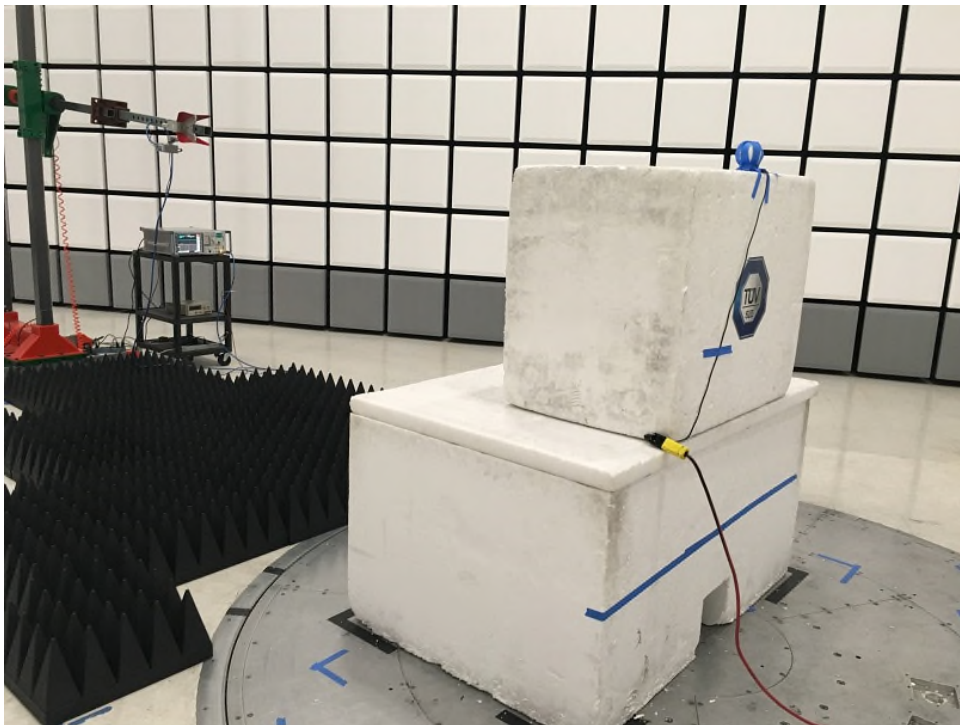
Radiated Spurious Emissions Above 1GHz 1GHz Rear (Baseball Transmit Mode)
