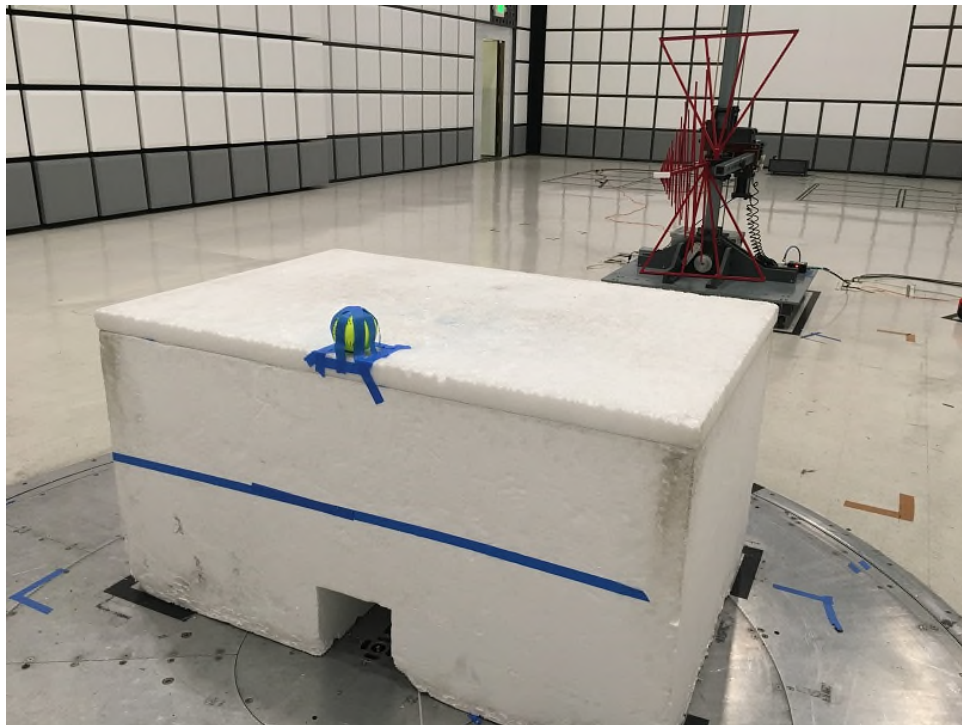
Radiated Spurious Emissions Below 1GHz Rear (Softball Transmit Mode)
