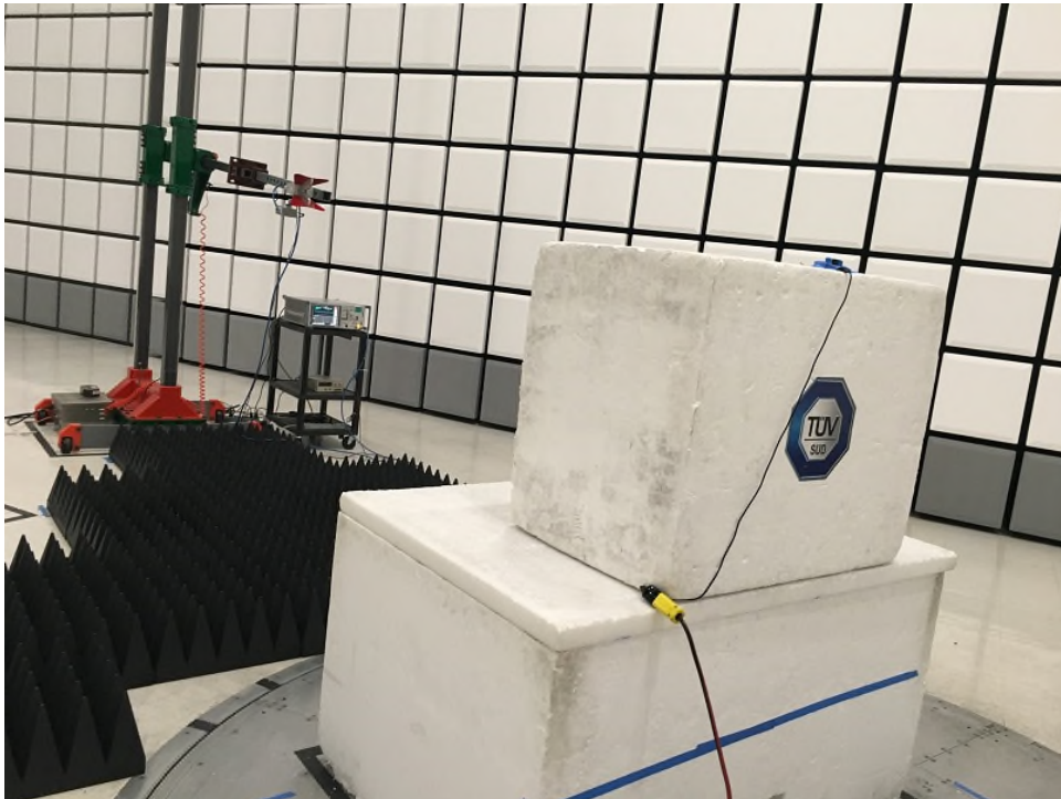
Radiated Spurious Emissions Above 1GHz 1GHz Rear (Swing tracker Transmit Mode)
