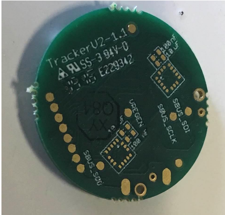
EUT – Internal view 4, PCB view 2
