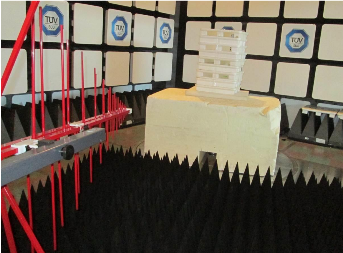
Test setup photo 3 Radiated measurements, 1 GHz – 2 GHz
