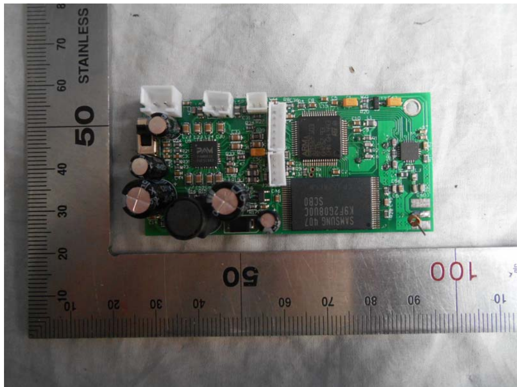
FIGURE 7 ELECTRONIC GAME CALLER (M/N: GS2BCALLER) MAIN BOARD (FRONT VIEW)
