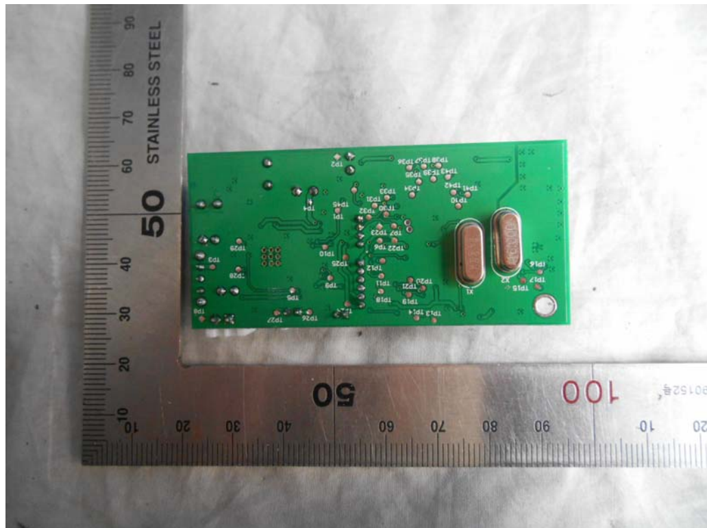
FIGURE 8 ELECTRONIC GAME CALLER (M/N: GS2BCALLER) MAIN BOARD (BACK VIEW)
