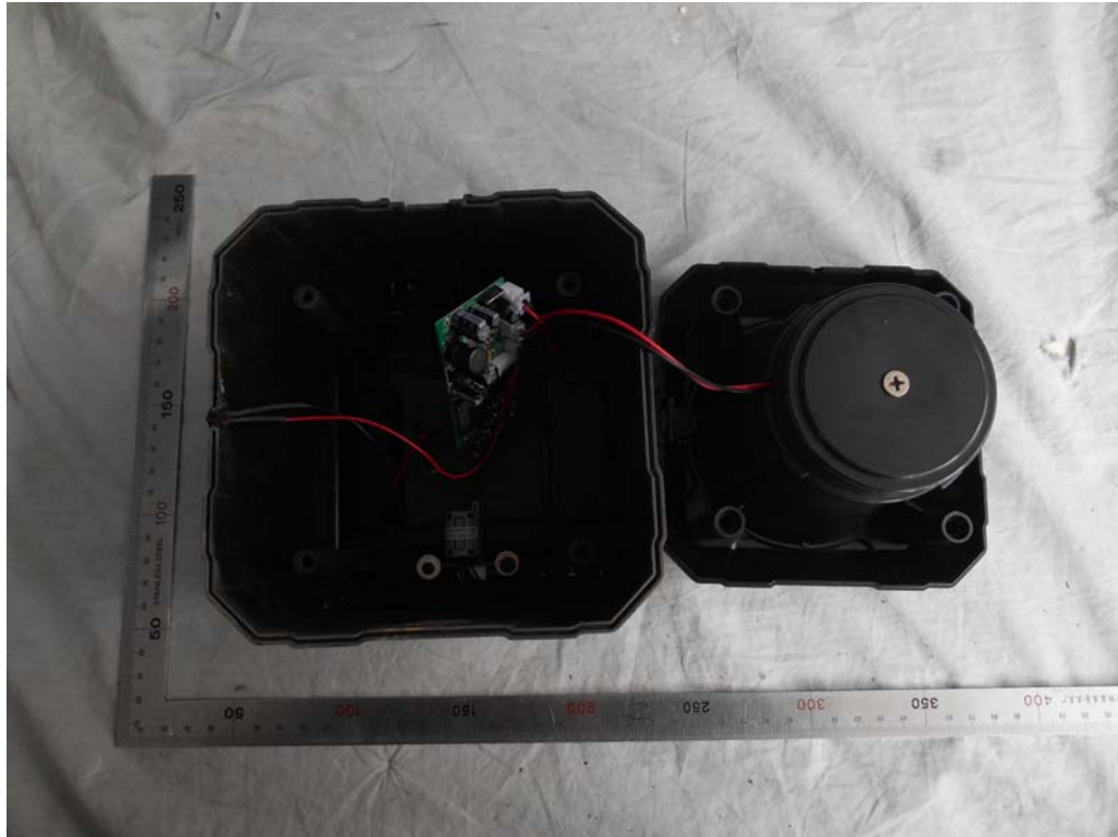
FIGURE 6 ELECTRONIC GAME CALLER (M/N: GS2BCALLER) COVER REMOVED
