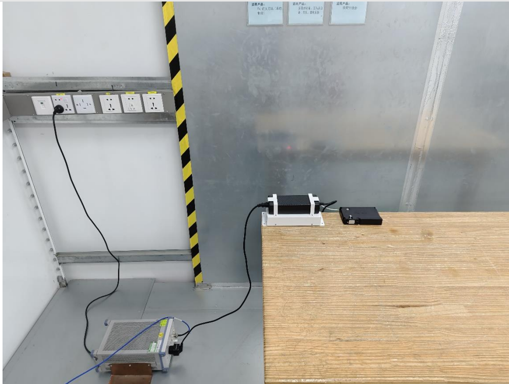
Radiated emissions 9K-30MHz
