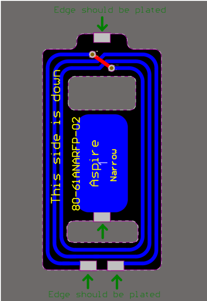
Trace Dimensions: 21.00mm x 39.5mm
