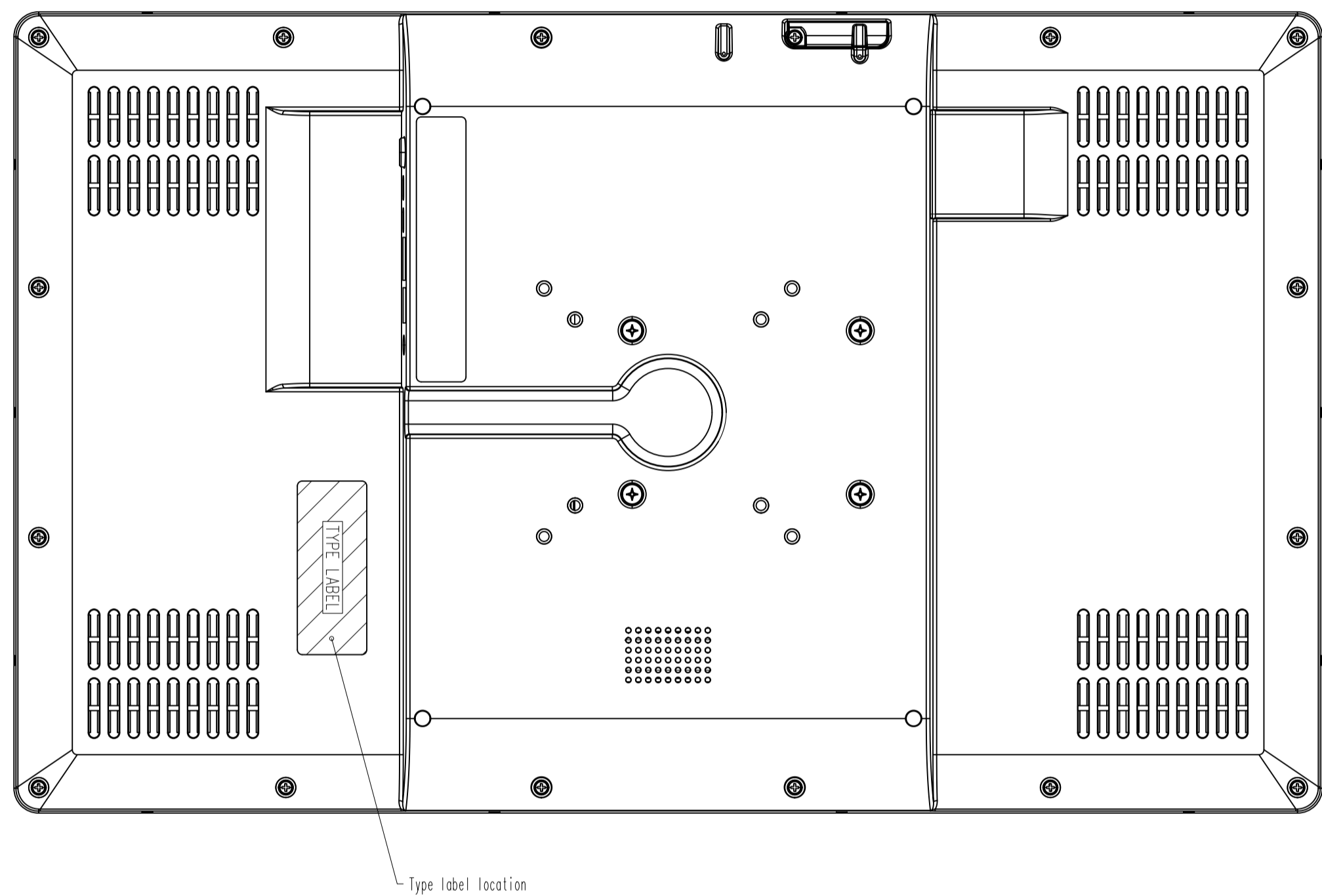
BACK VIEW
