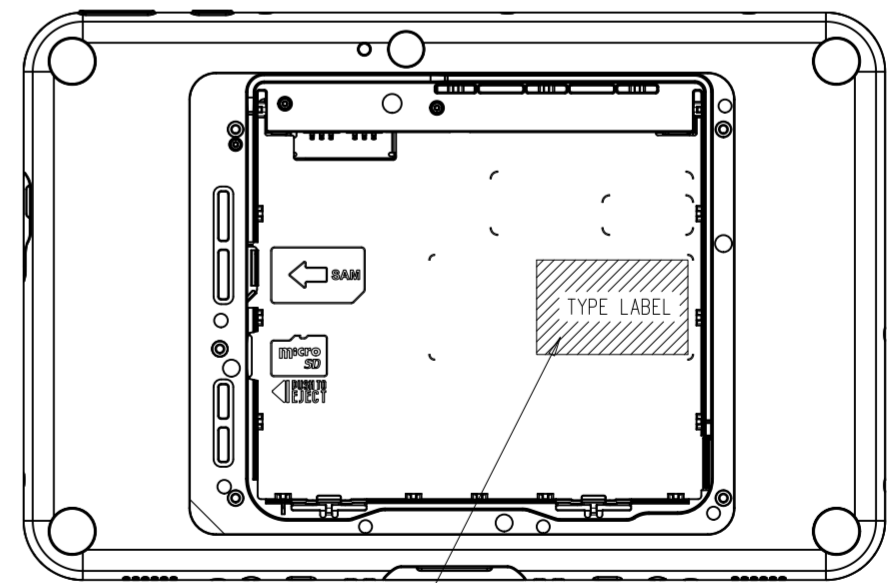
BACK VIEW Without battery cover and battery
