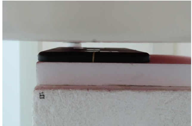
Bottom Face, Test Separation 14 mm
