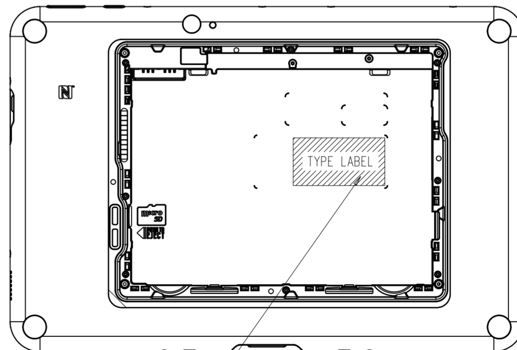
BACK VIEW without battery cover and battery
