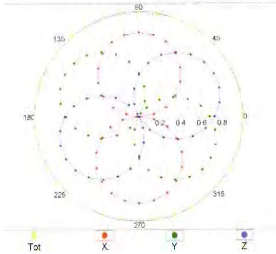
f=600 MHz,TEM
