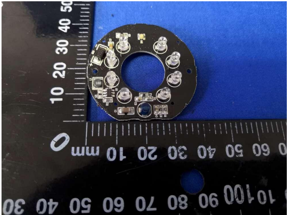
LED-Front View(SVC562)
