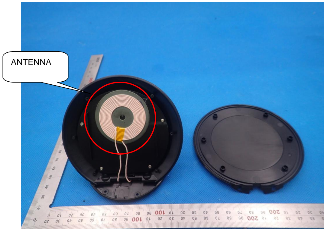
OPEN VIEW-2 OF EUT
