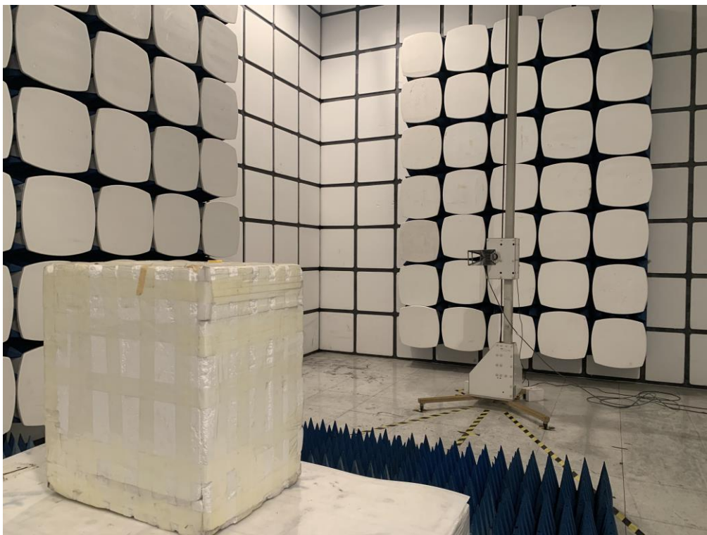
Spurious Emission Test Setup (Above 1GHz)
