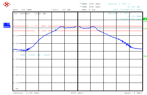
Middle 0.687MHz
