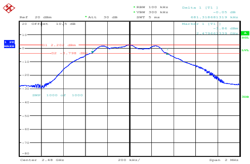
High 0.681MHz
