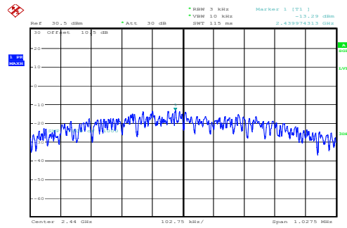
Middle -13.29dBm/3kHz
