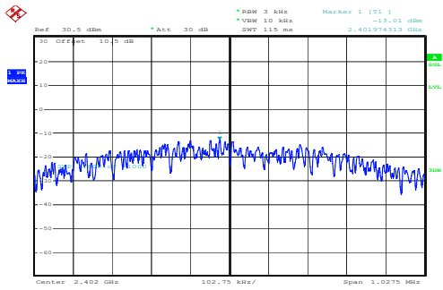
Low -13.01dBm/3kHz
