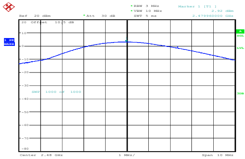
High 2.92dBm
