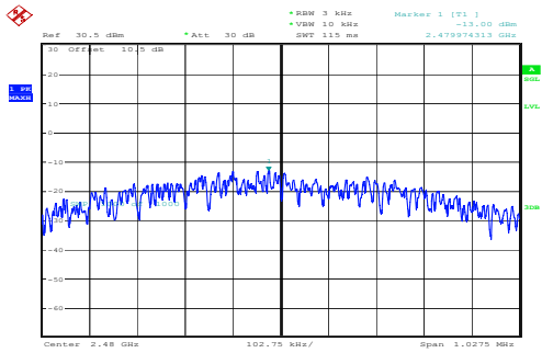
High -13.00dBm/3kHz
