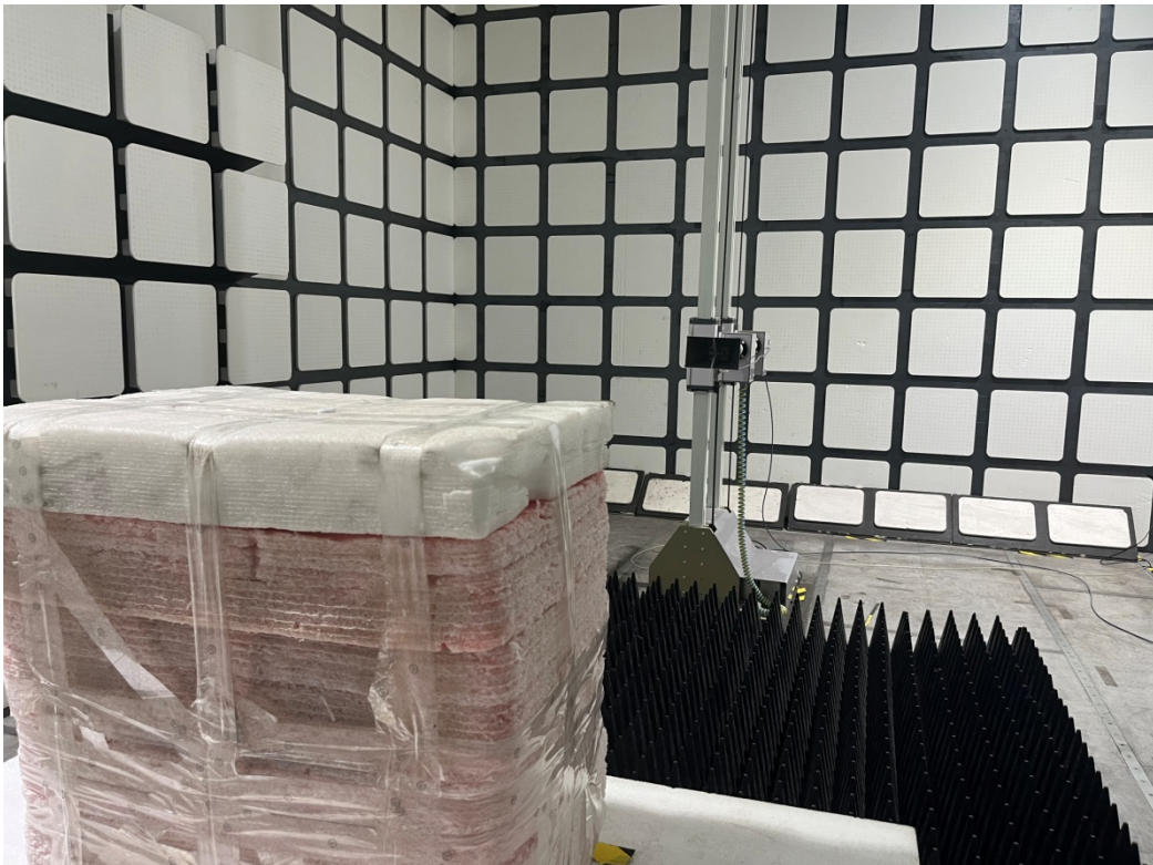
Radiated Emission View (1-18 GHz)
