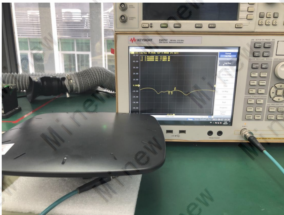
S11
