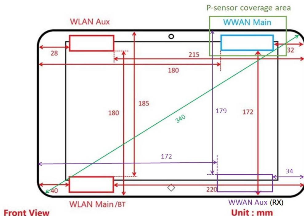
Fig.12 Antenna position of EUT
