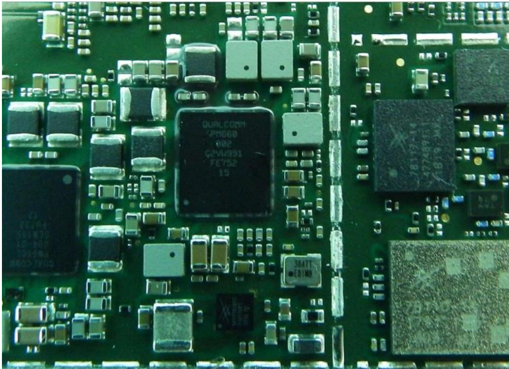
(7) EUT Photo
