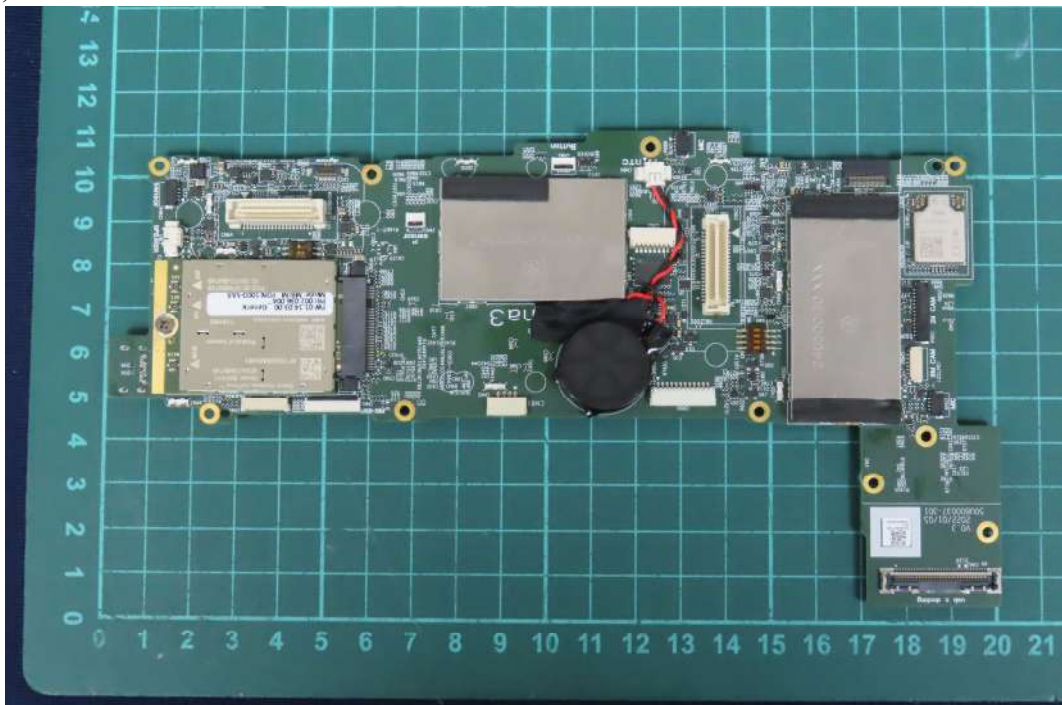
(32) EUT Photo
