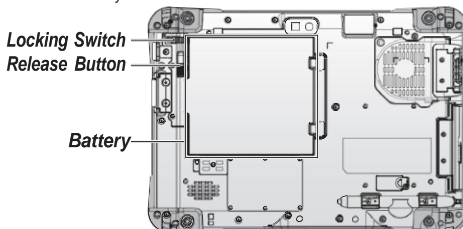
Figure 41. Rear View: Locating the Battery
