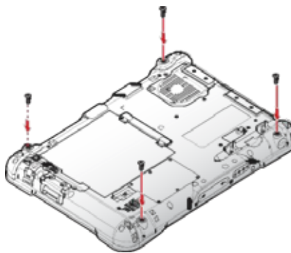
Figure 33. Securing the Screws
