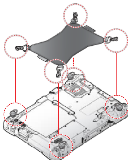
Figure 30. Connecting the Handstrap
