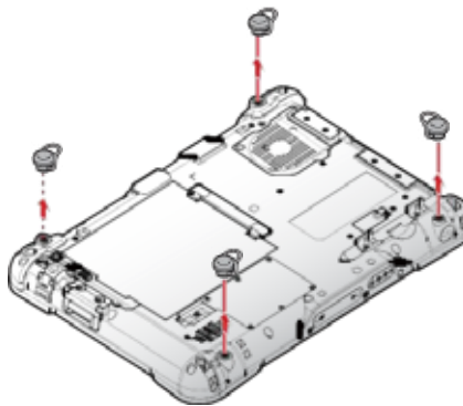
Figure 32. Removing the D-rings
