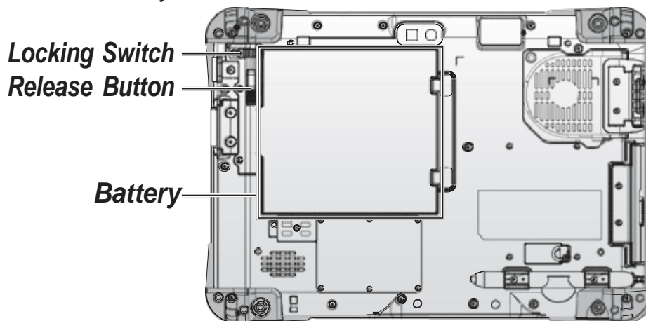
Figure 38. Rear View: Locating the Battery
