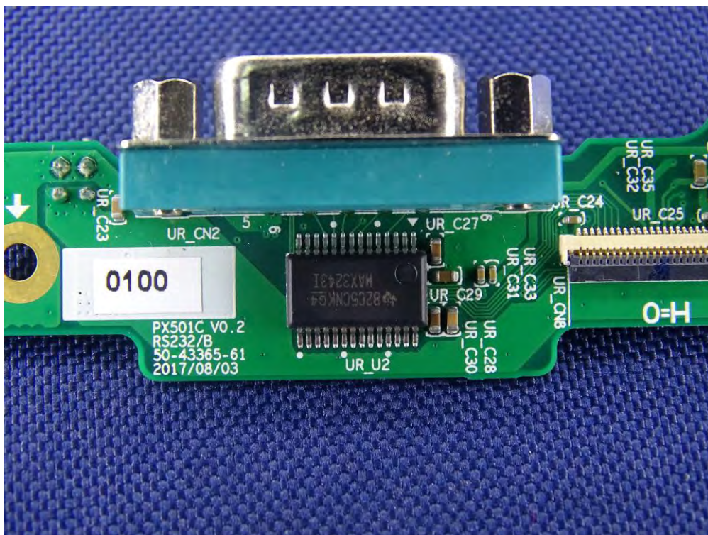
(28) EUT Photo
