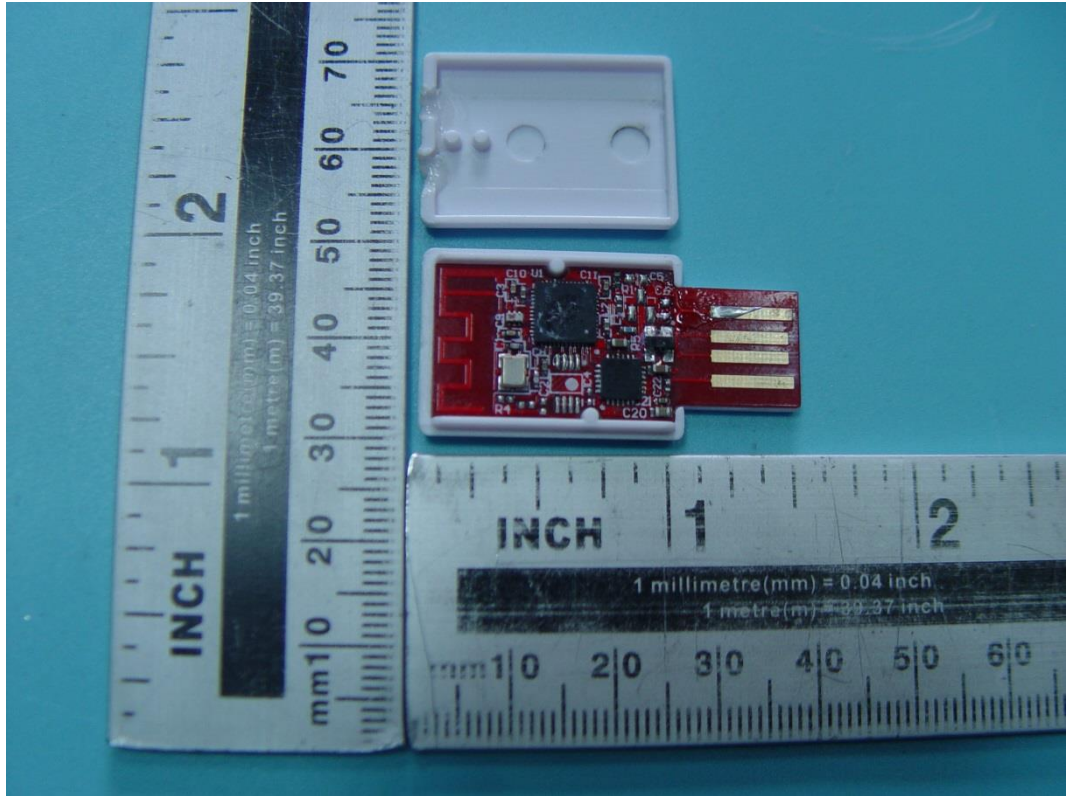
Fig. 1: Internal view
