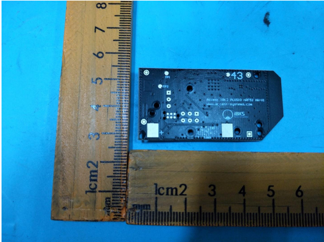
Fig. 7: Main board bottom view
