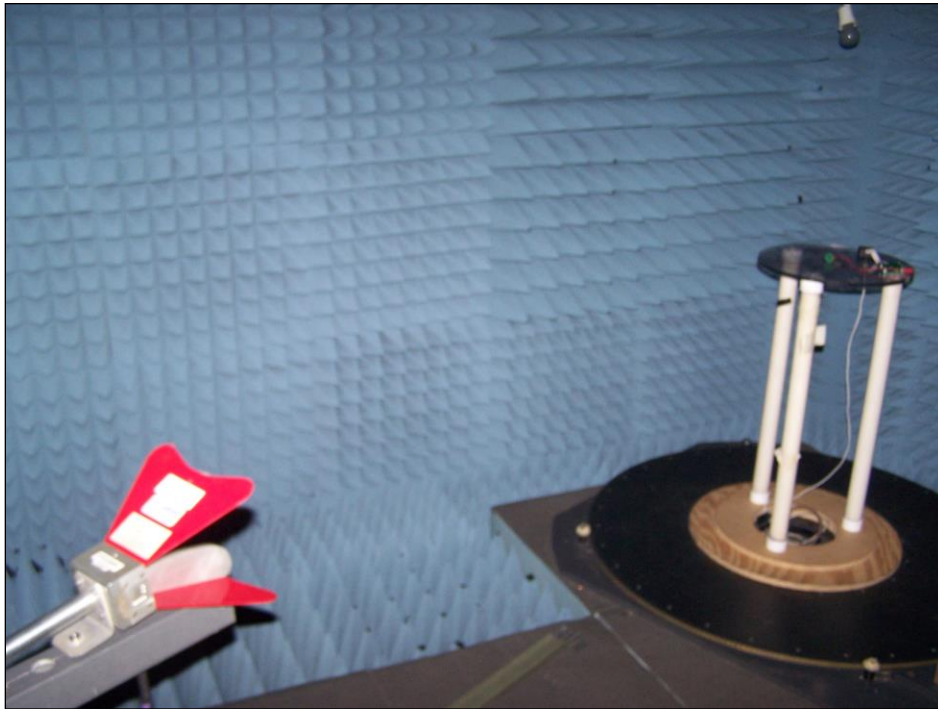
Photograph 3. Radiated Spurious Emissions, 1GHz-18GHz, Test Setup
