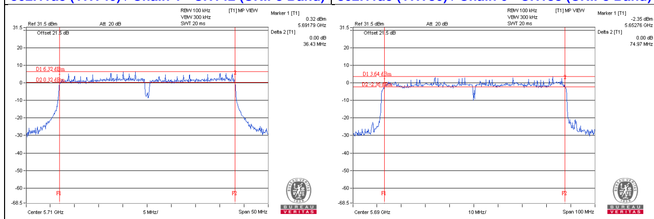
802.11ac (VHT40) / Chain 1 - CH142 (UNII-3 Band)
