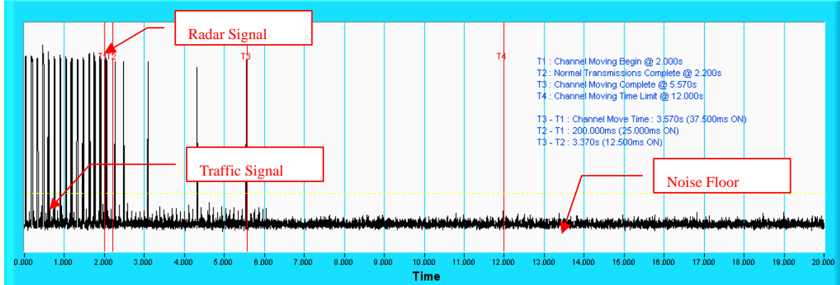
Channel Closing Transmission Time & Channel Move Time @ AC80-106
