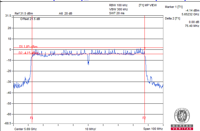
802.11ac (VHT80)_Chain 2 / CH138 (U-NII-3)
