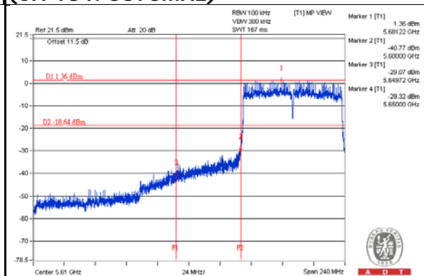
802.11ac (VHT80) MODULATION (CH 138: 5690MHz)
