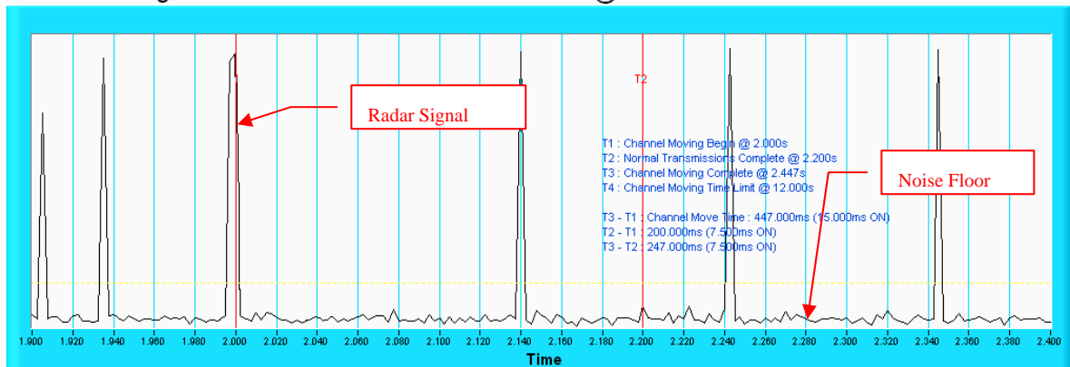
Channel Closing Transmission Time & Channel Move Time @ ac80 - ch106
