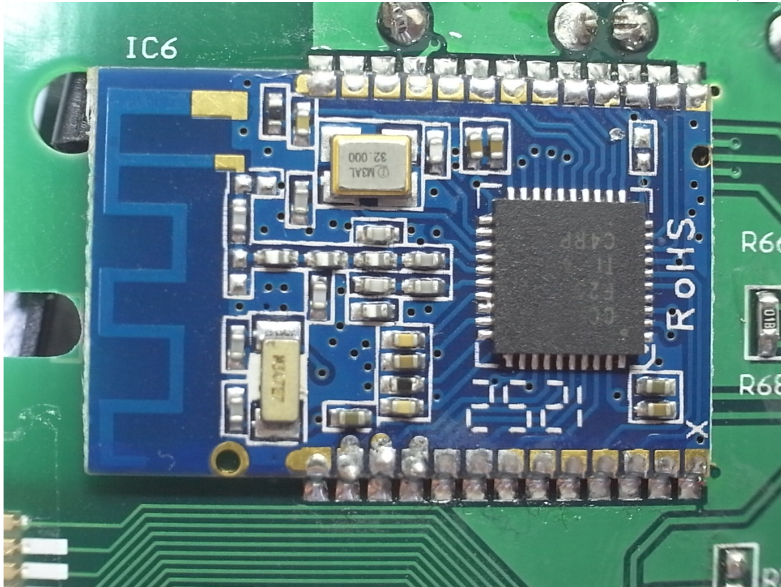
Figure 9 Internal View (BT Module, Front View)
