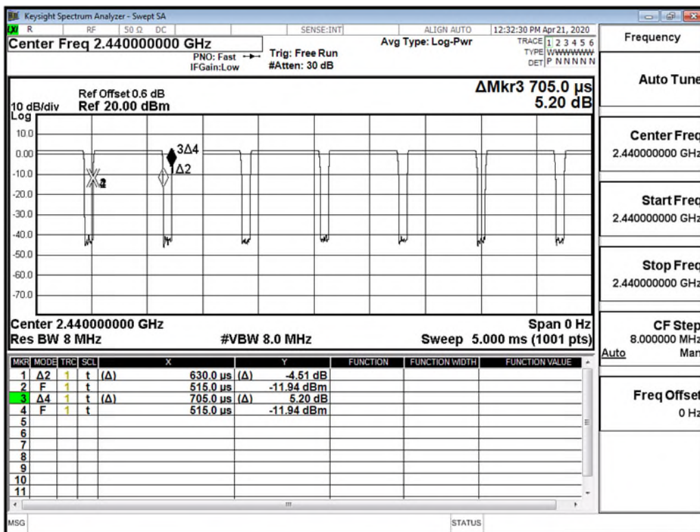
Duty Cycle_BLE_1M_MidCH19-2440
