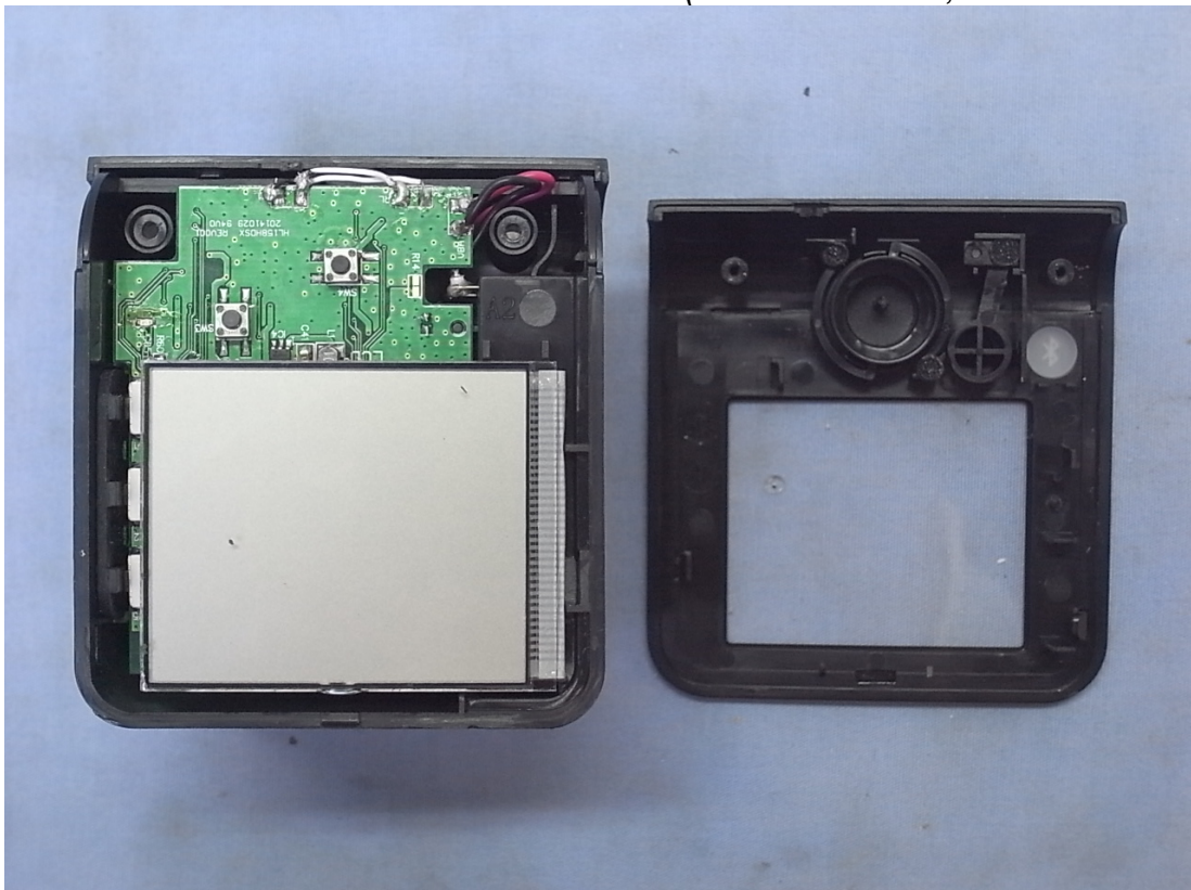
Figure 4 Internal View (Removed Cover, LCD Panel/Front View)
