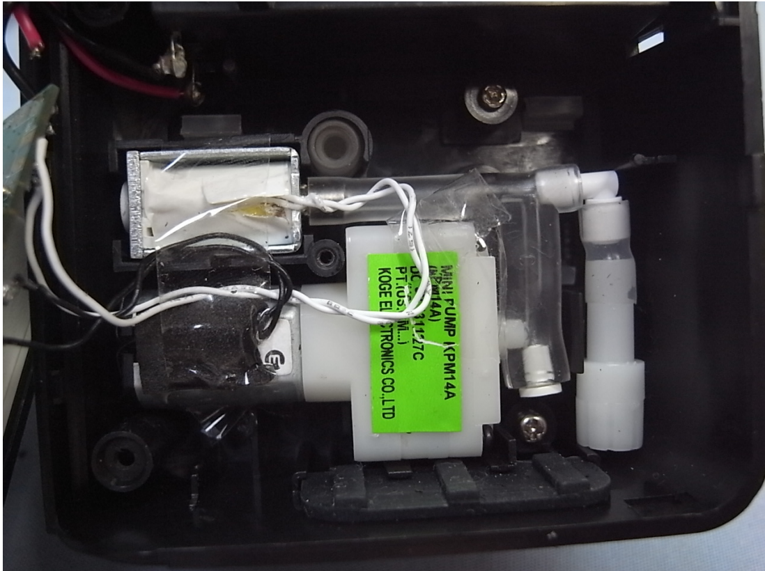
Figure 10 Internal View
