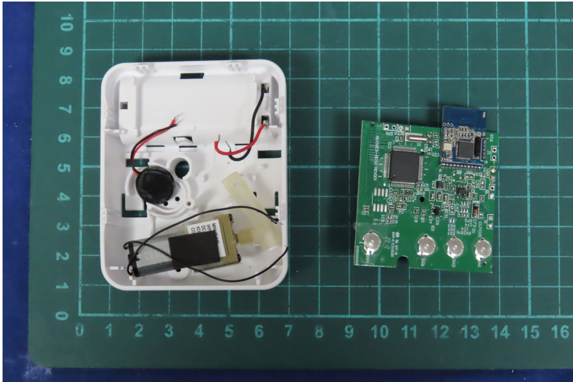
(7) EUT Photo
